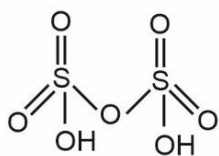
Pyrosulphuric acid ( \text{H}_2\text{S}_2\text{O}_7 )
